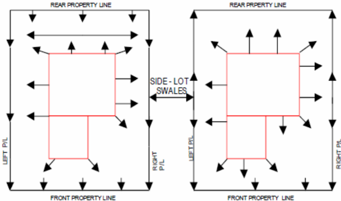
REAR TO FRONT SURFACE DRAINAGE
